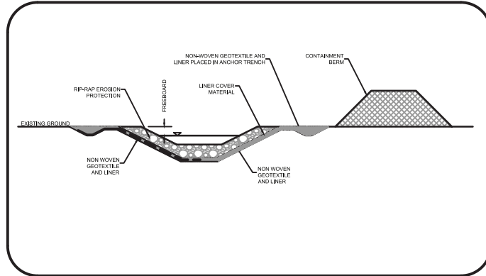
RUNOFF COLLECTION DITCH TYPE B-1 RUNOFF AND SEEPAGE COLLECTION
