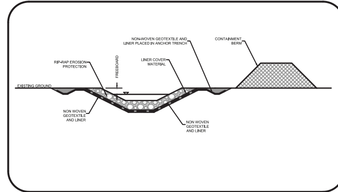
RUNOFF COLLECTION DITCH TYPE B-1 RUNOFF COLLECTION AND TRANSPORTATION TO COLLECTION PONDS
