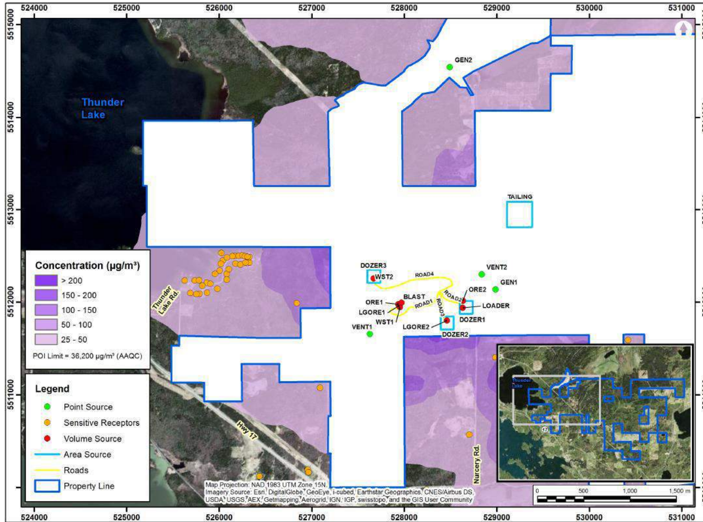
Figure 13: CO 1hr Contour Plot (criteria: 36,200 µg/m³)
