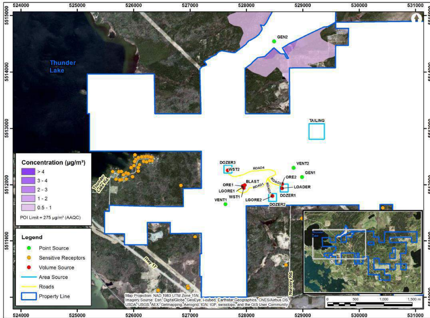
Figure 18: SO 2 24hr Contour Plot (criteria: 275 \mu\text{g}/\text{m}^3 )
