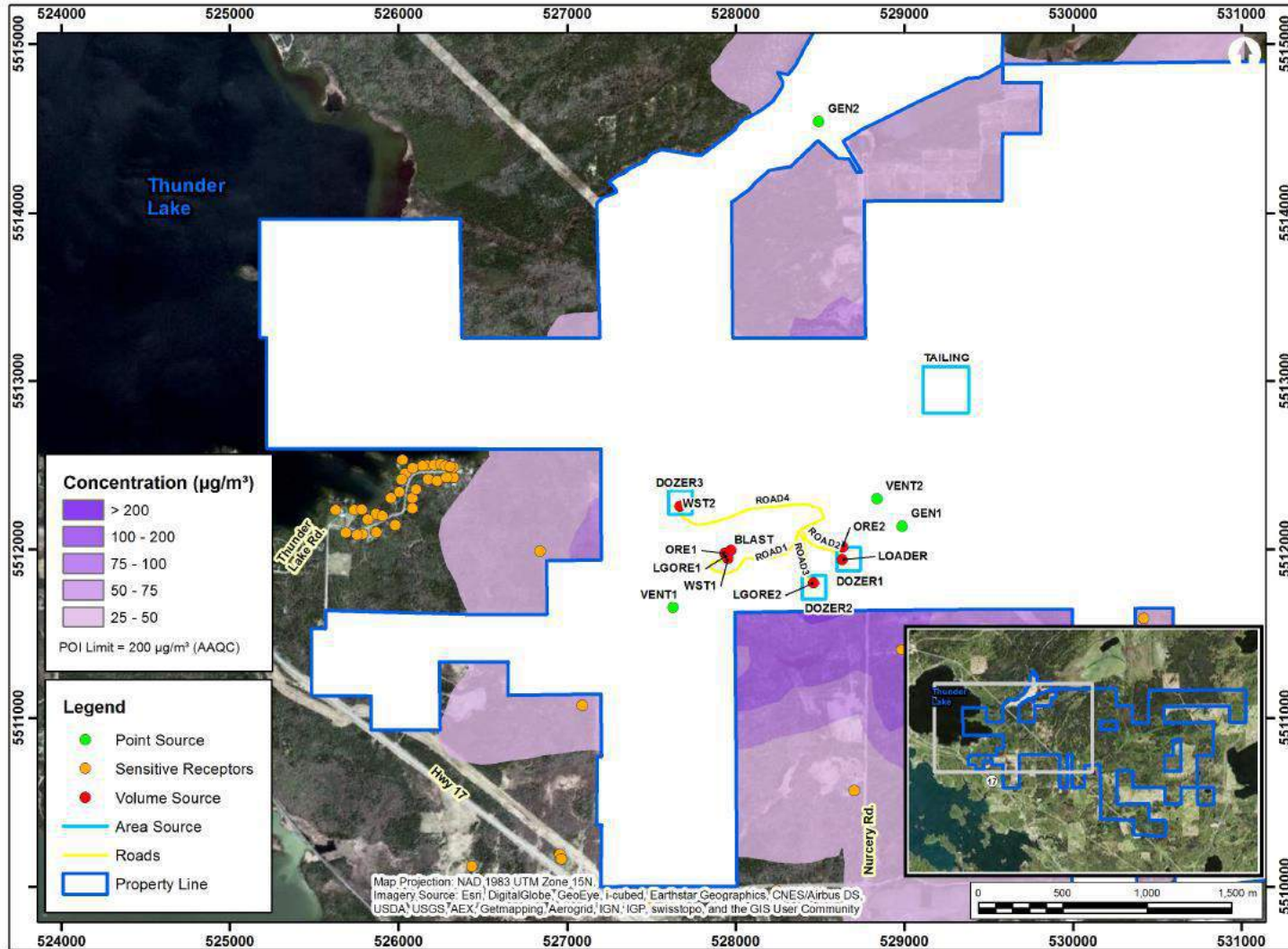
Figure 16: NO 2 24hr Contour Plot (criteria: 200 µg/m 3 )
