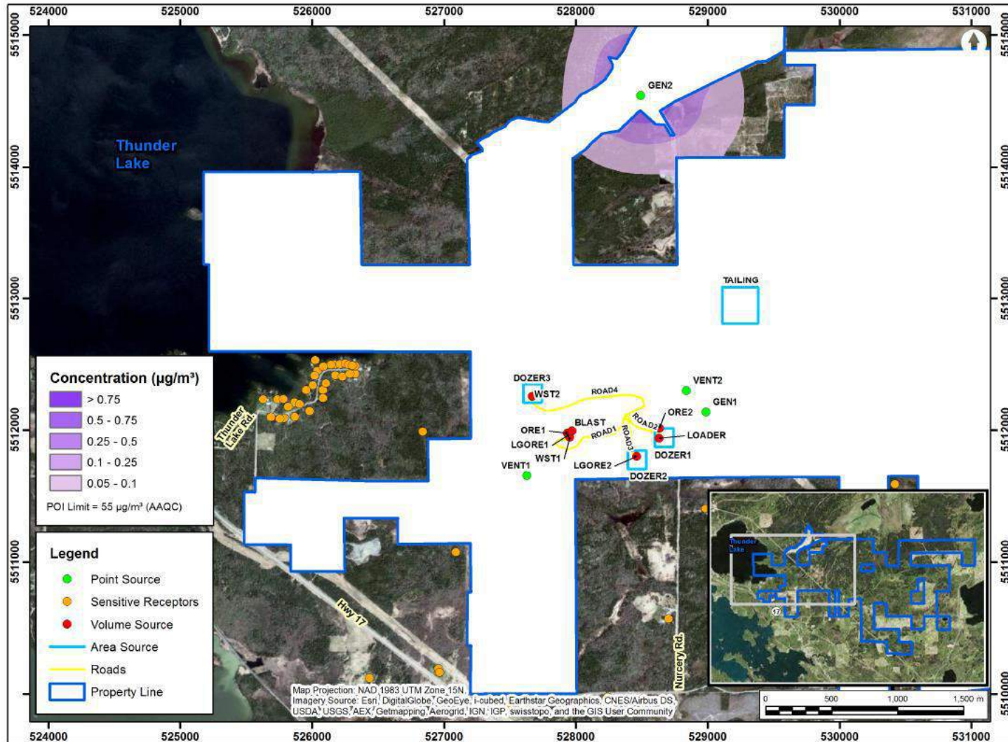
Figure 19: \text{SO}_2 Ann Contour Plot (criteria: 55 \mu\text{g}/\text{m}^3 )
