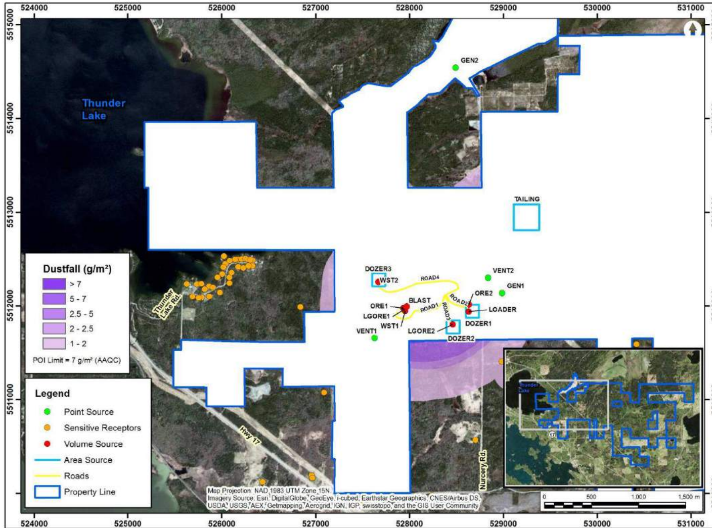
Figure 11: Dustfall 30 day Contour Plot (criteria: 7 g/m²/30 days)
